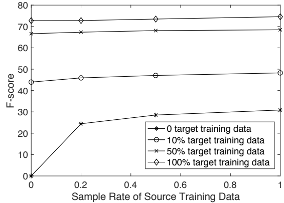
Figure 4: The impact of the size of annotations from source and target languages on Amharic name tagging.
