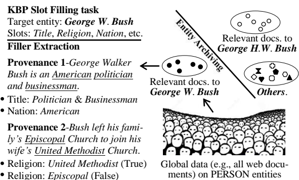
Figure 1: Use of entity archiving in slot filling
